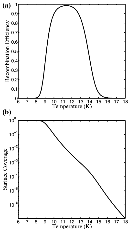
Figure 6. (a) Calculated recombination efficiency and surface coverage (b) of hydrogen on the amorphous silicate sample vs surface temperature, under steady-state conditions. A temperature window of high efficiency is found. Within this window, the surface coverage is reduced from a full monolayer to about 10^{-4} ML.
