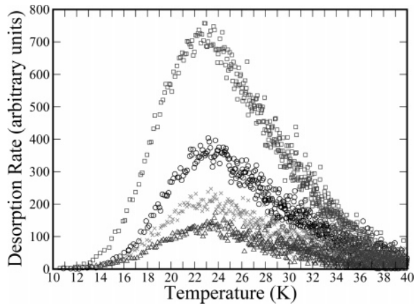
Figure 4. TPD traces obtained after irradiation with H + D atoms at a sample temperature of 10 K. The irradiation times are 30 (triangles), 60 ( \times ), 120 (circles), and 240 (squares) seconds.
