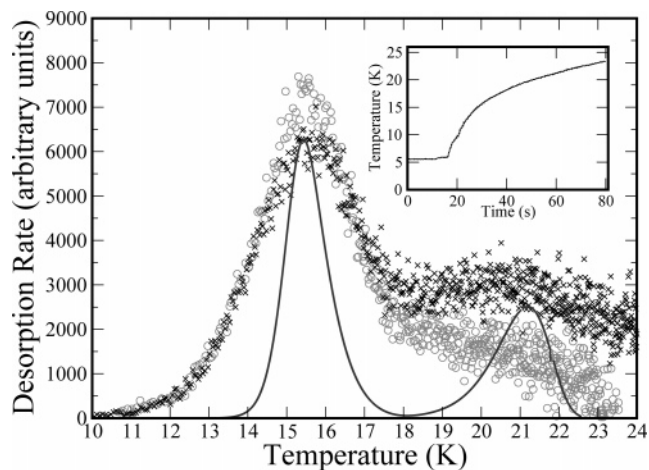
Figure 1. TPD curves of HD desorption after irradiation H + D atoms (circles) and HD molecules ( \times ) on the amorphous silicate sample at surface temperature of 5.6 K. The fit of the TPD curve for H + D irradiation, obtained using the rate equations, is also shown (solid line). The temperature ramp T(t) during the TPD stage is shown in the inset.
