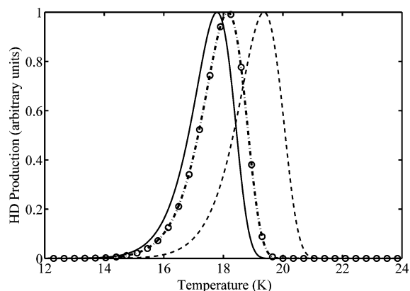
Figure 5. Simulated TPD curves of HD production and desorption obtained from eqs 1, following irradiation by H + D atoms at 5.6 K and heating at a constant rate of 0.5 K/s. In this figure, it is assumed that HD molecules desorb upon formation. Four choices of parameters are shown: the parameters of H and D are identical and are given by Table 1 (solid line); the desorption energy barrier of D is raised by 4.0 meV (dashed-dotted line); both the desorption and diffusion energy barriers of D are raised by 4.0 meV (circles); the desorption and diffusion energy barriers of both H and D are raised by 4.0 meV (dashed line). The results indicate that the higher binding energy of D atoms has little effect on the TPD curves. The peak heights are normalized to 1, to make it easier to compare the peak locations.
