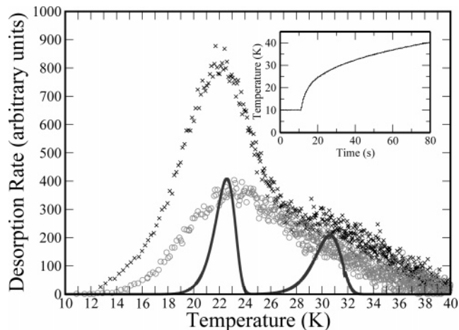
Figure 2. TPD curves of HD desorption after irradiation H + D atoms (circles) and HD molecules ( \times ) on the amorphous silicate sample at surface temperature of 10 K. The fit of the TPD curve for H + D irradiation, obtained using the rate equations, is also shown (solid line). The temperature ramp T(t) during the TPD stage is shown in the inset.
