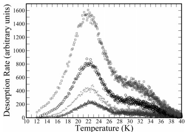
Figure 3. TPD traces obtained after irradiation with HD molecules at a sample temperature of 10 K. The irradiation times are 30 (triangles), 60 ( \times ), 120 (circles), and 240 (squares) seconds.
